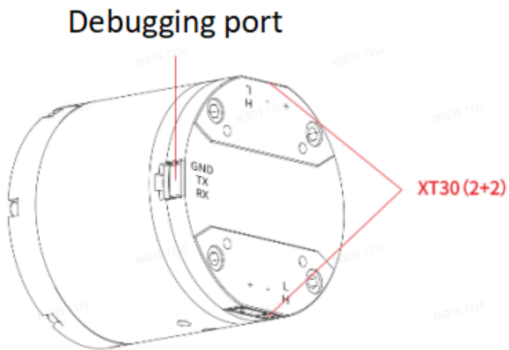
Radial cable exit XD5757-1
