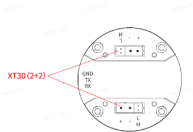
Axial cable exit XD5757-2
